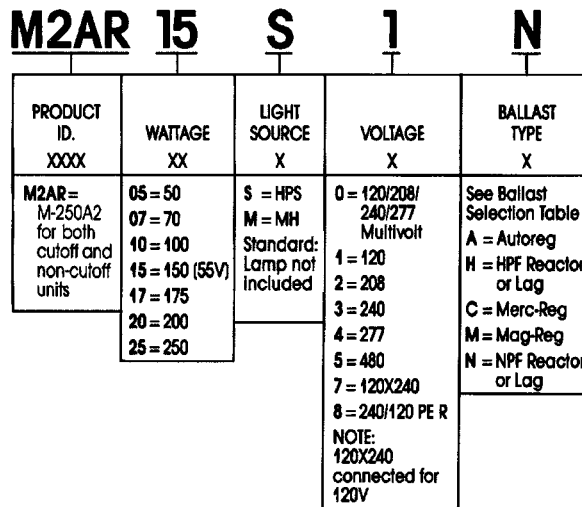
BALLAST SELECTION TABLE
