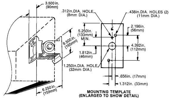
KNUCKLE FLAT SURFACE ADAPTER UTILIZES SAME BOLT PATTERN AS STANDARD MOUNTING ARM
