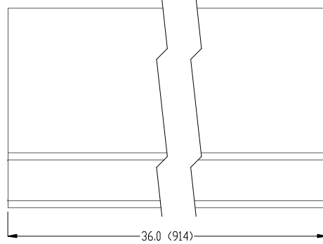
AL10 Mounting Track with Shield
