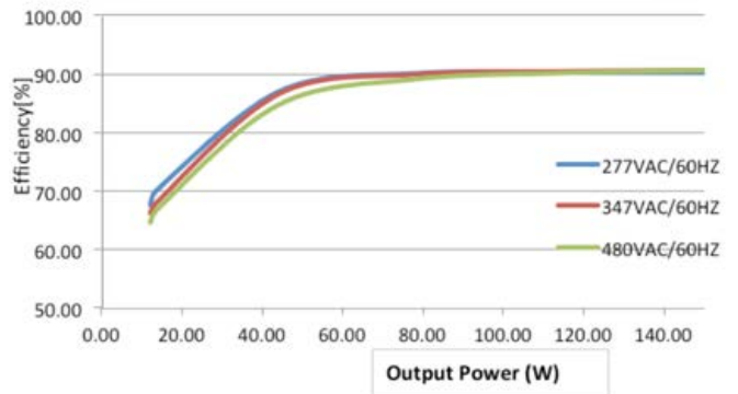
Efficiency vs. Output Power
