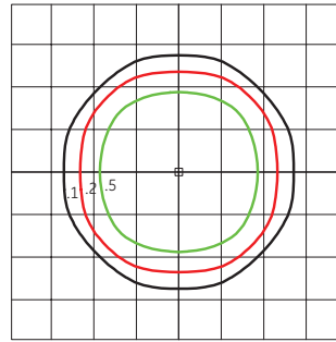
EALS Type V - Symmetric Wide (U5) 31,000 Lumens, 5000K (EALS02_U5SW750____.IES)
