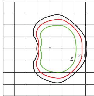
EALS Type III - Asymmetric Wide (K3) 31,000 Lumens, 5000K (EALS02_K3AW750____.IES)
