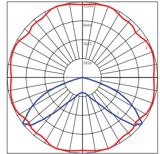
EALS Type V - Symmetric Wide (U5) 31,000 Lumens, 5000K (EALS02_U5SW750____.IES)
