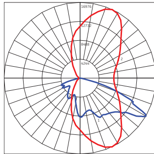
EALS Type II - Asymmetric Narrow (K2) 30,500 Lumens, 5000K (EALS02_K2AN750____.IES)
