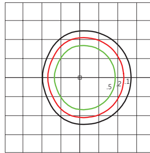
EALS - Assymmetric Auto (KA) 34,200 Lumens, 5000K (EALS02_KAAA750____.IES)
