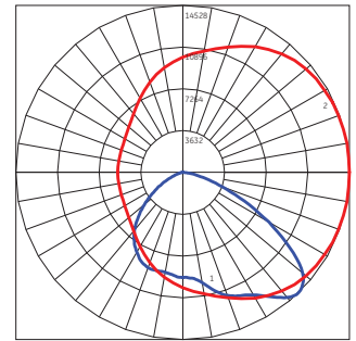
EALS - Assymmetric Auto (KA) 34,200 Lumens, 5000K (EALS02_KAAA750____.IES)
