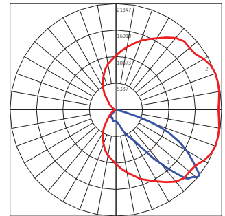
EALS Type III - Asymmetric Wide (K3) 31,000 Lumens, 5000K (EALS02_K3AW750____.IES)
